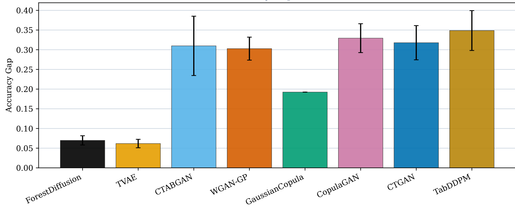
Forest Cover — Accuracy Gap (mean \pm SD, 10 seeds)
